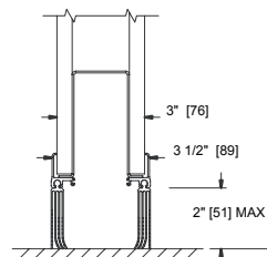
Optional: Bottom continuous contact (sweep) seals
