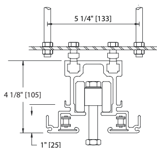
Type 42 Track with optional suspension bracket for 5-1/4" [133] spacing.
