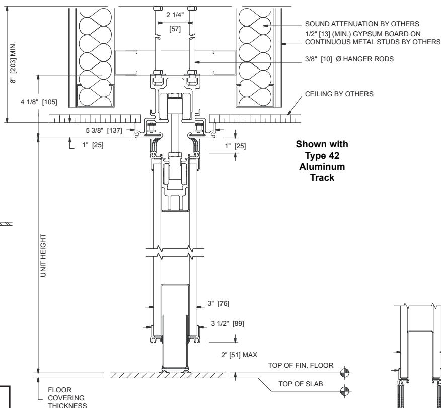
Optional: Bottom continuous contact (sweep) seals
